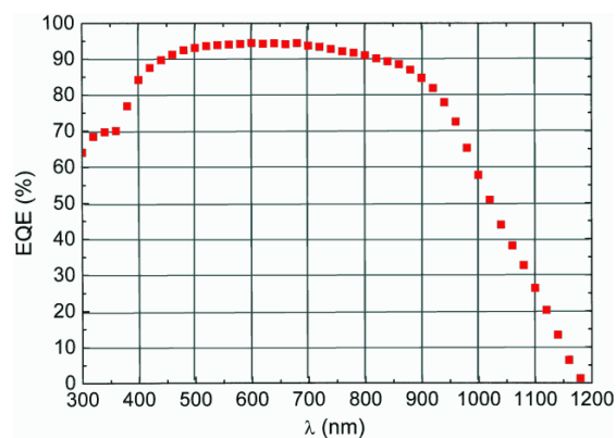
External Quantum Efficiency
